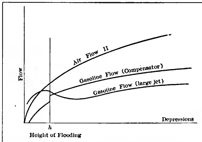
Fig. 8—Showing the flow from the large and compensating jets of the Claudel carburetor, together with the air flow
